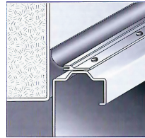
Top Weatherstrip Vinyl header-seal at top
