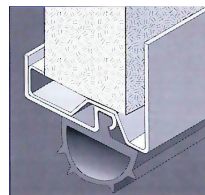
Bottom Weatherstrip Full-length bottom PVC weatherstrip for superior air-right seal (Standard feature)
